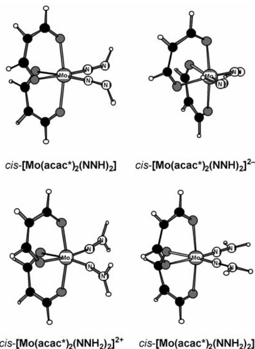
Fig. 5 Optimized geometries of the models cis\text{-}[\text{Mo}(\text{acac}^*)_2(\text{NNH})_2]^{0/2-} and cis\text{-}[\text{Mo}(\text{acac}^*)_2(\text{NNH}_2)_2]^{2+/0} . \text{acac}^* = [\text{HC}(=\text{O})\text{CHC}(=\text{O})\text{H}]^- .
