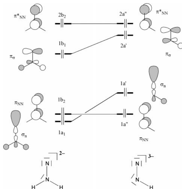
Fig. 1 The frontier orbitals of the C_{2v} \text{NNH}_2^{2-} (left) and C_s \text{NNH}_3^{3-} (right) planar ligands. The anionic charges are purely arbitrary (see text).
